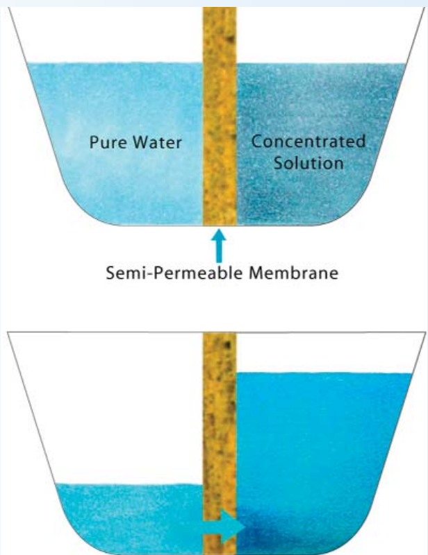
The drawing shows that pure water with no salts or dissolved solids migrates to the solution with more dissolved solids.
